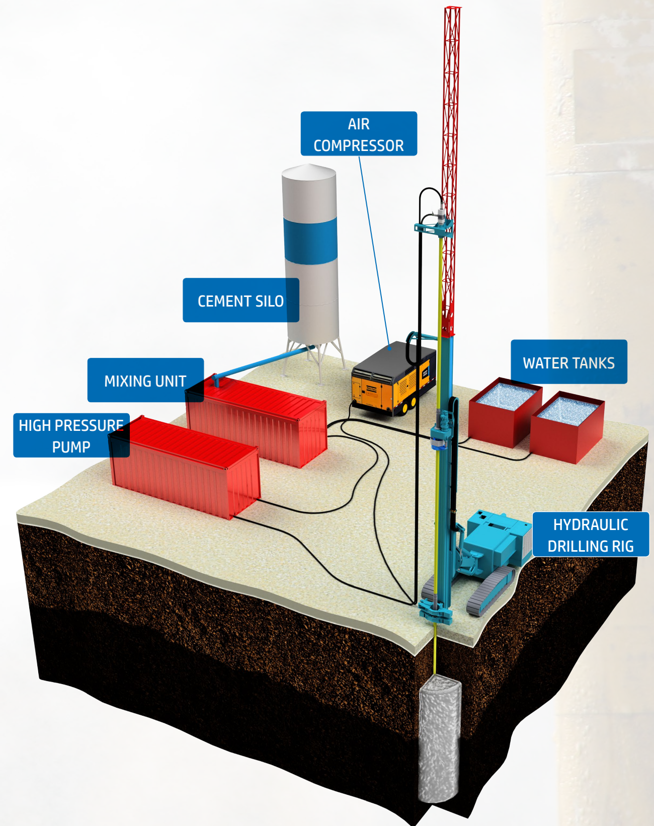
DOUBLE FLUID JET GROUTING PLANT - SCHEMA IMPIANTO JET GROUTING BIFLUIDO
