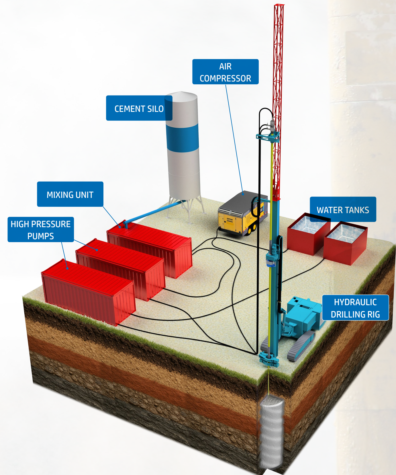
TRIPLE FLUID JET GROUTING PLANT - SCHEMA IMPIANTO JET GROUTING TRIFLUIDO
