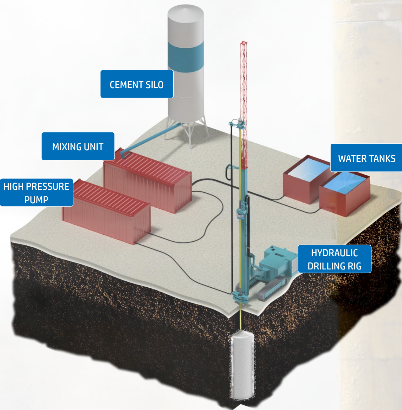
SINGLE FLUID JET GROUTING PLANT - SCHEMA IMPIANTO JET GROUTING MONOFLUIDO
